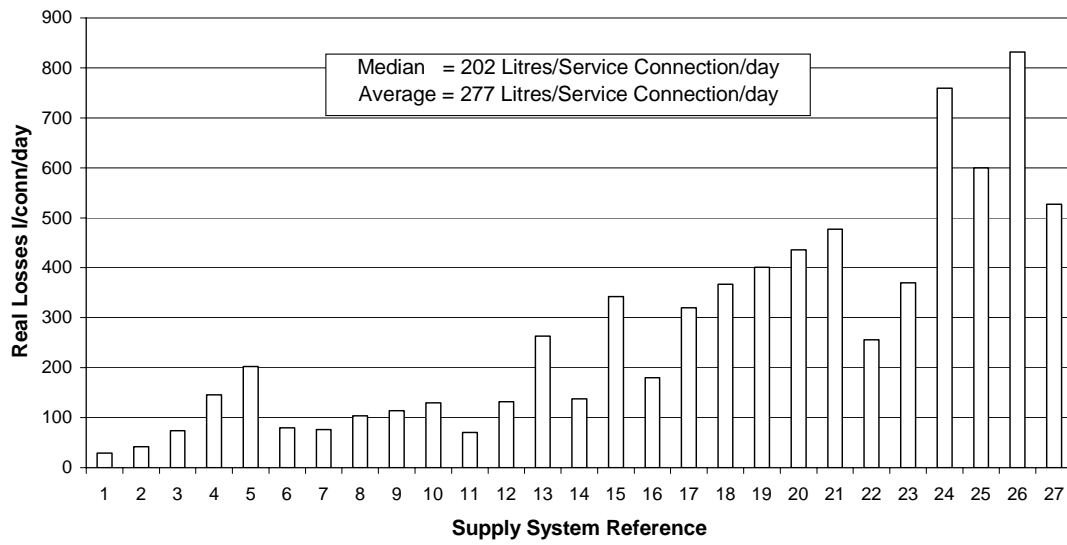
Figure 1: Technical Indicator for Real Losses (TIRL) in Litres/Service Connection/day for 27 Water Supply Systems from 20 Countries
