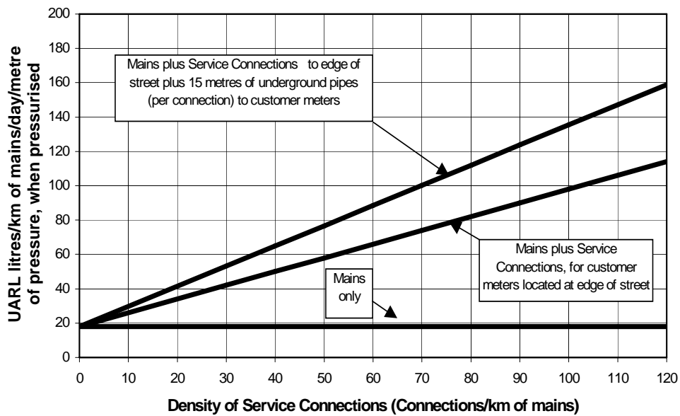
Figure 5: Unavoidable Annual Real Losses in Litres per Km of Mains per day per Metre of Pressure, vs Density of Service Connections
